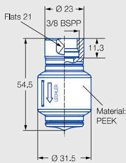
Standard version Female thread 59x.xx9.1Y.AF
